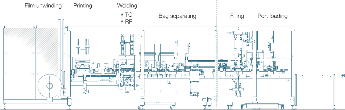
Example: Form-Fill-Seal machine
